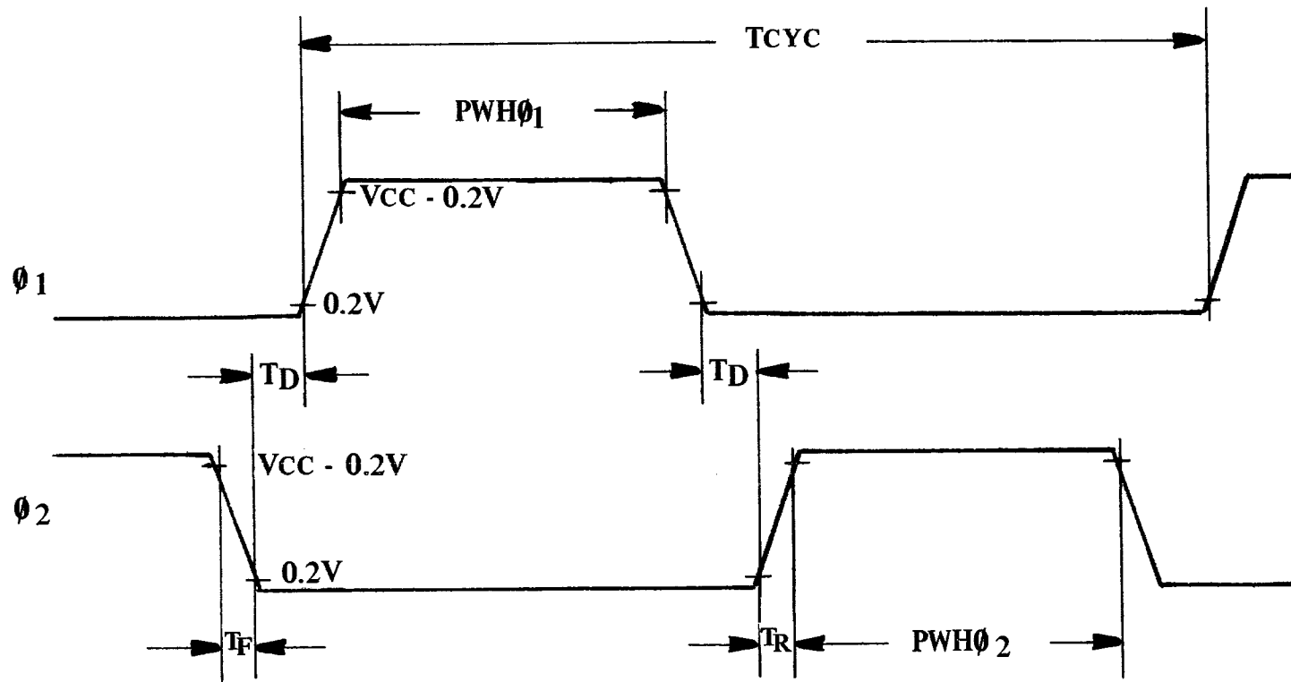
Two Phase Clock Timing
